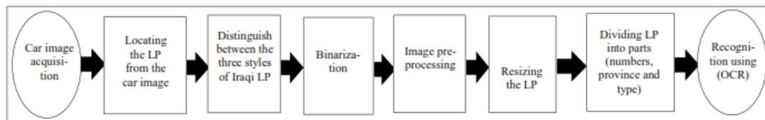
Fig. 3. The main stages of the LPR system
