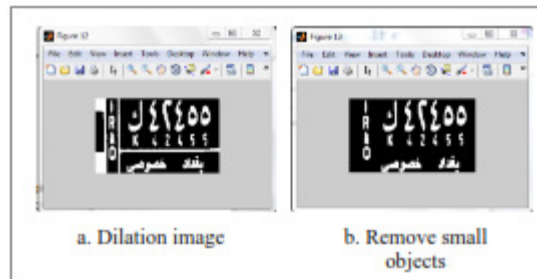
Fig. 9. Image pre-processing
